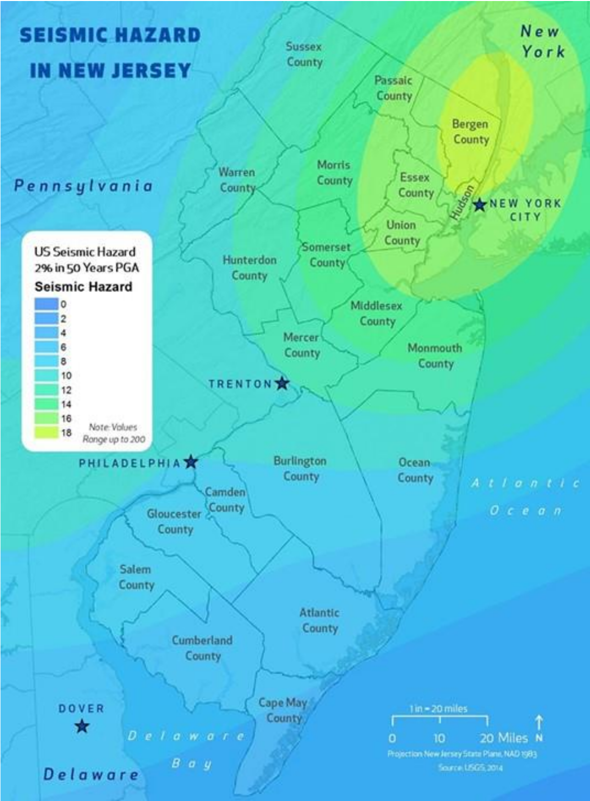
Figure 4.7-1 Seismic Hazard for New Jersey
