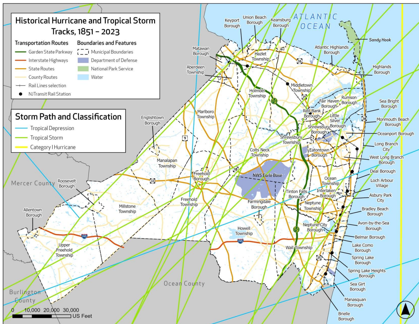
Figure 4.11-1 Historical Hurricane and Tropical Storm Tracks, 1851 – 2023
