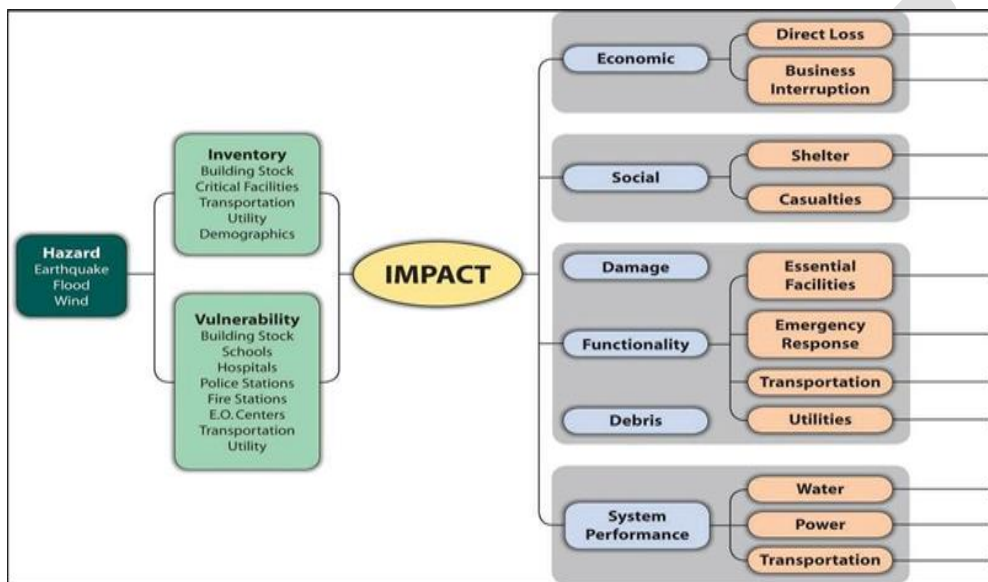
Figure 4.3-1 Conceptual Model of HAZUS-MH Methodology
