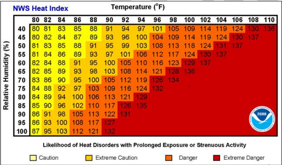
Figure 4.8-2 NWS Heat Index
