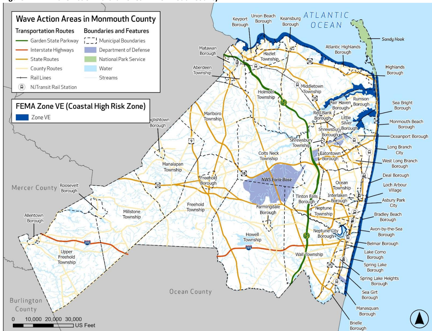
Figure 4.17-2 Wave Action Hazard Zones in Monmouth County
