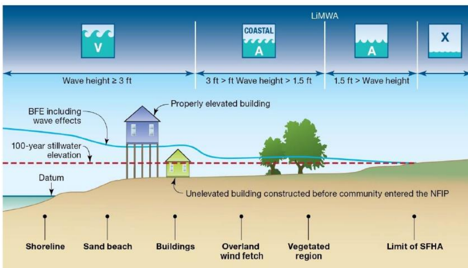
Figure 4.17-1 Transect Schematic of Zone V, Coastal A-Zone and Zone A
