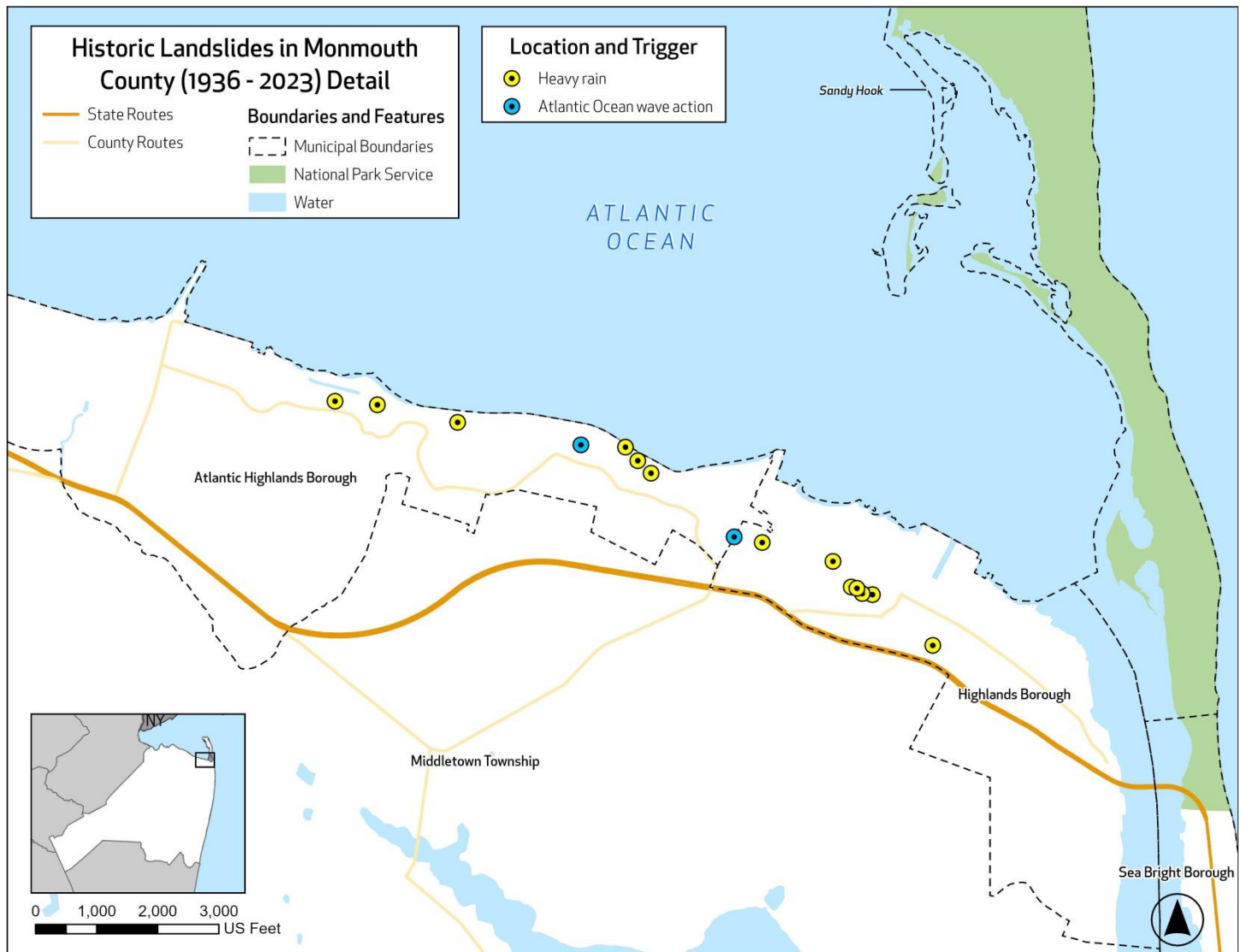
Figure 4.12-2 Previous Occurrences of Landslides in Monmouth County and their Triggers (Detail)
