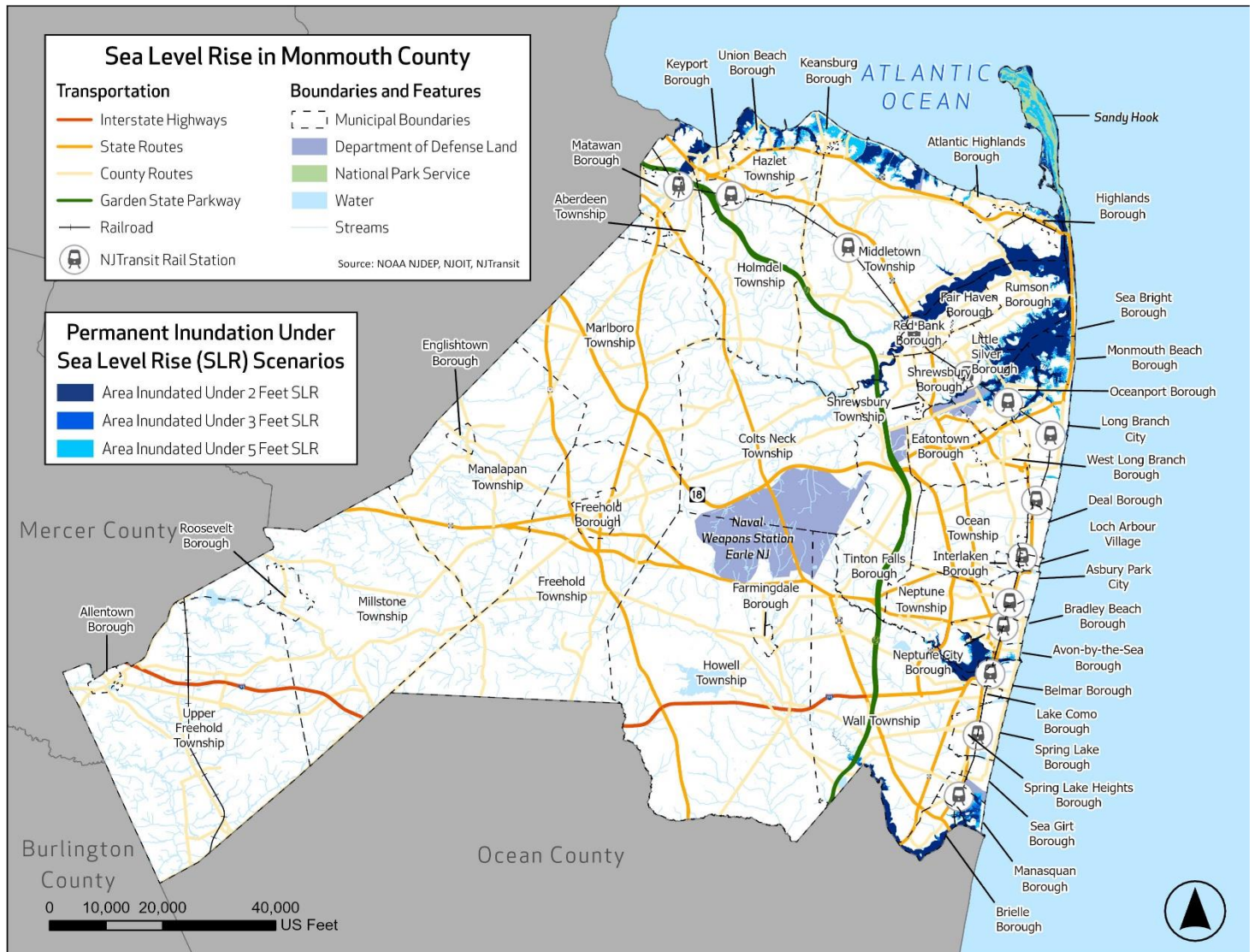
Figure 4.10-3 Permanent Inundation Under Sea Level Rise Scenarios in Monmouth County
